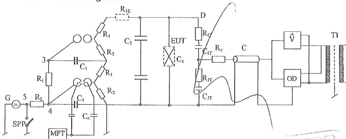
Fig. 3 - Circuit diagram
